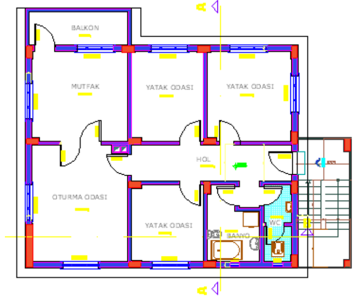
1. NORMAL KAT PLANI Ö:1/50
