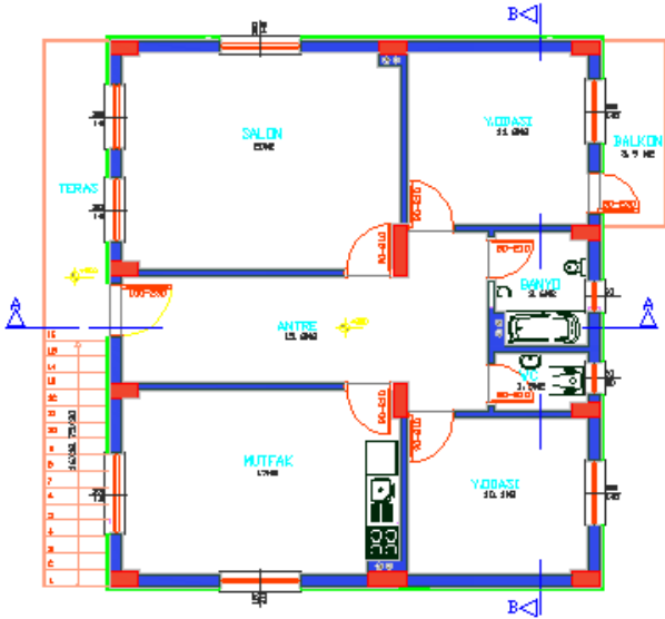
1. NORMAL KAT PLANI Ö:1/50
