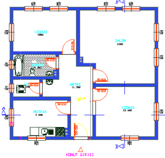
TADİLATLI ZEMİN KAT PLANI Ö:1/50
