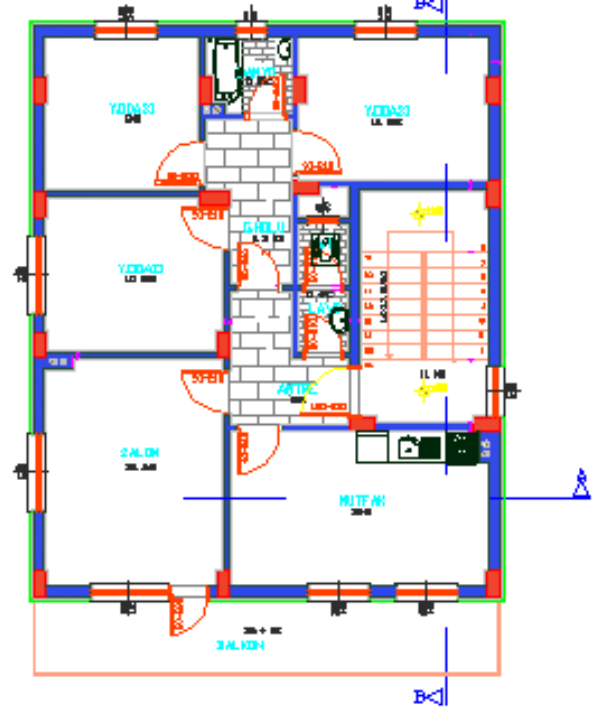
1. NORMAL KAT PLANI Ö:1/50
